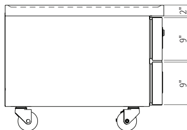
Side Section
